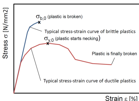
Figure A.7.2: typical stress strain curve of ductile plastics and brittle plastics
