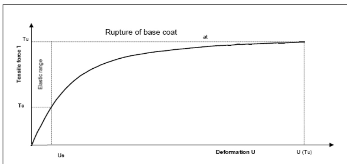
Figure 4: Load/displacement curve
