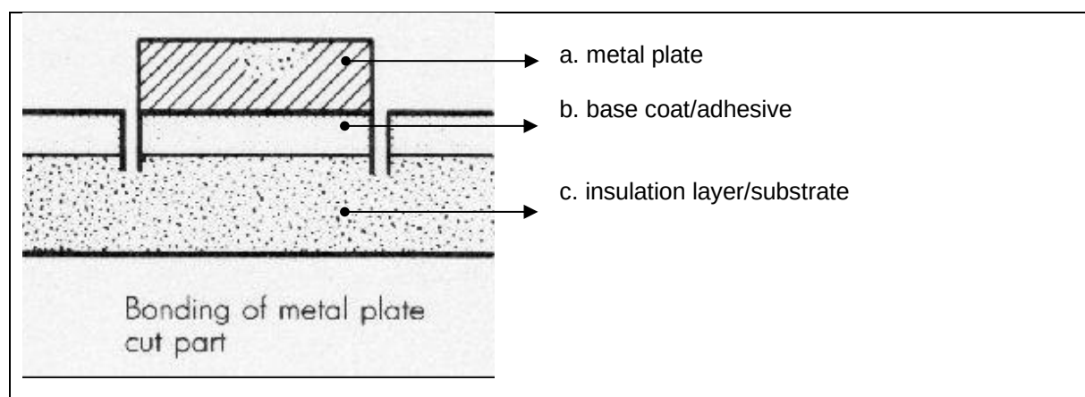
Figure 2: Pull-off test
